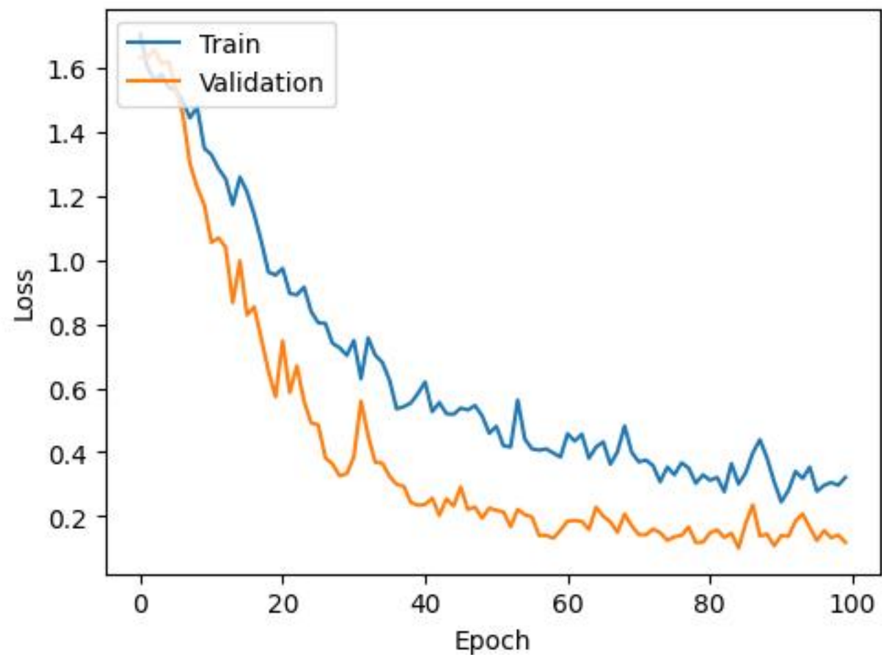
Model Loss
