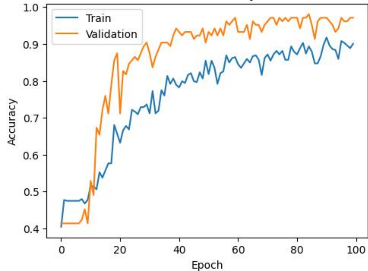
Model Accuracy
