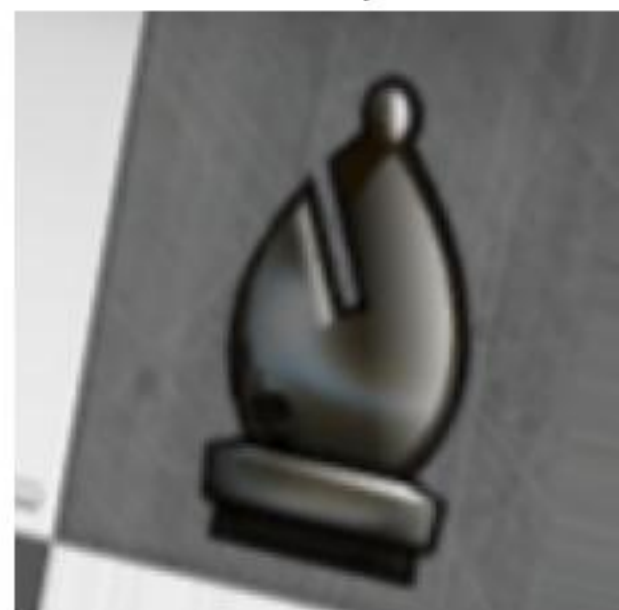
bishop
