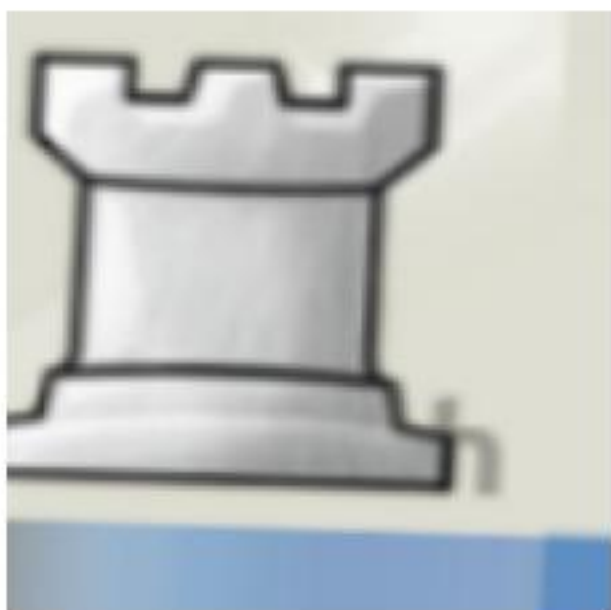
rook
