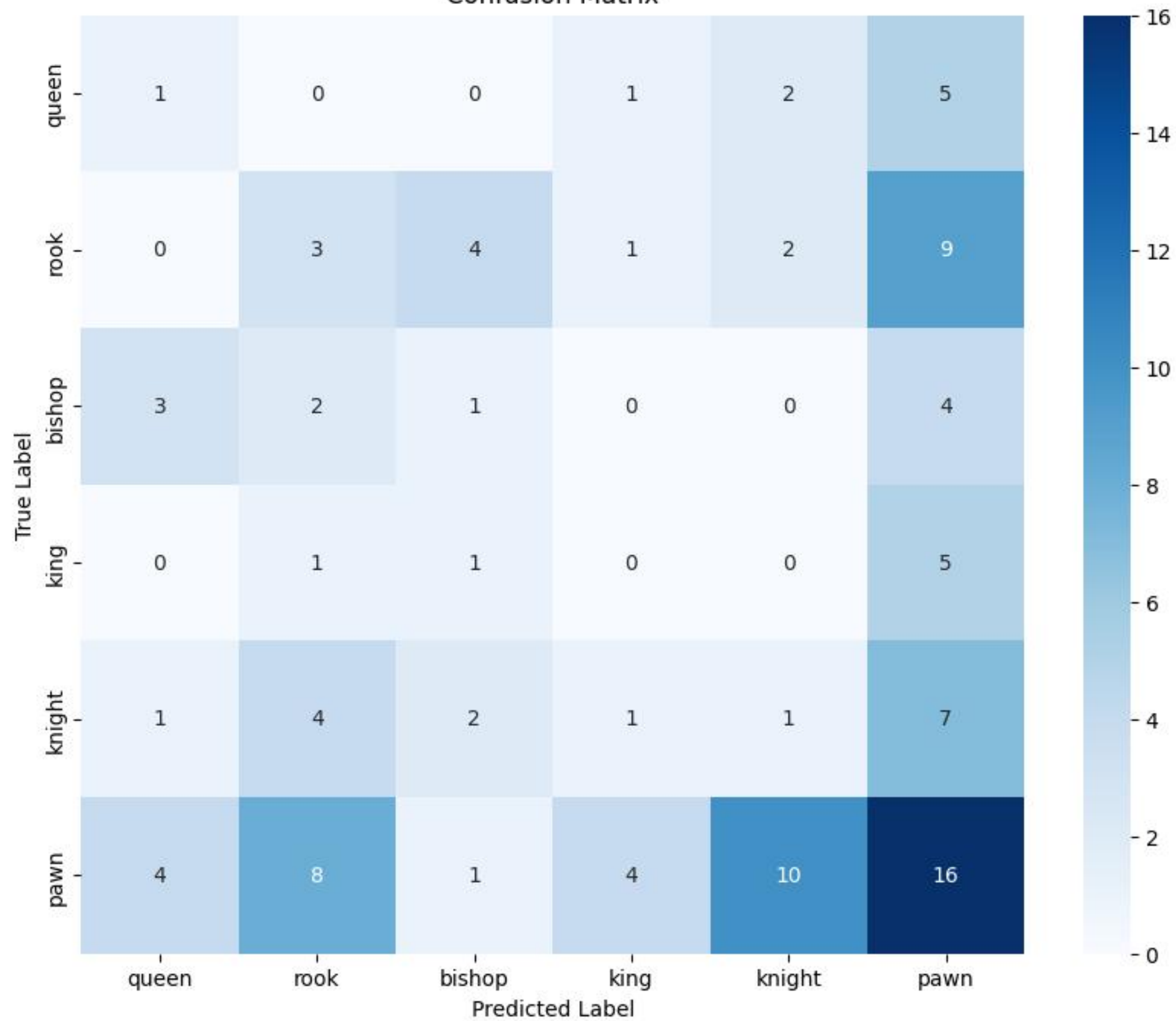
Confusion Matrix
